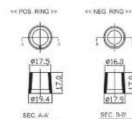
Ring Adaptors
